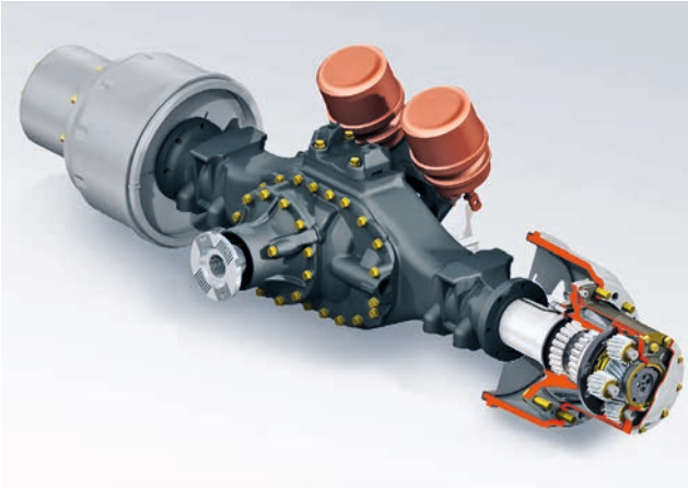
Planetary axle
