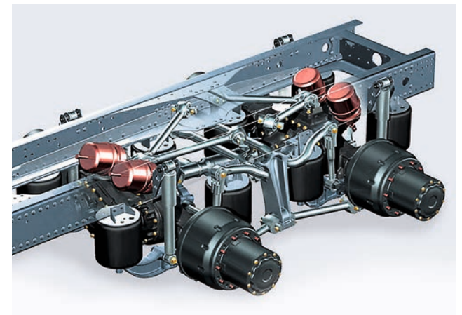
Construction air suspension
